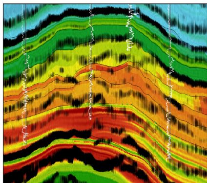
Well QC showing predicted facies, facies probabilities and synthetic-seismic comparisons
