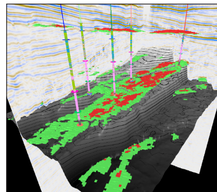
Hydrocarbon bodies from a Ji-Fi inversion
