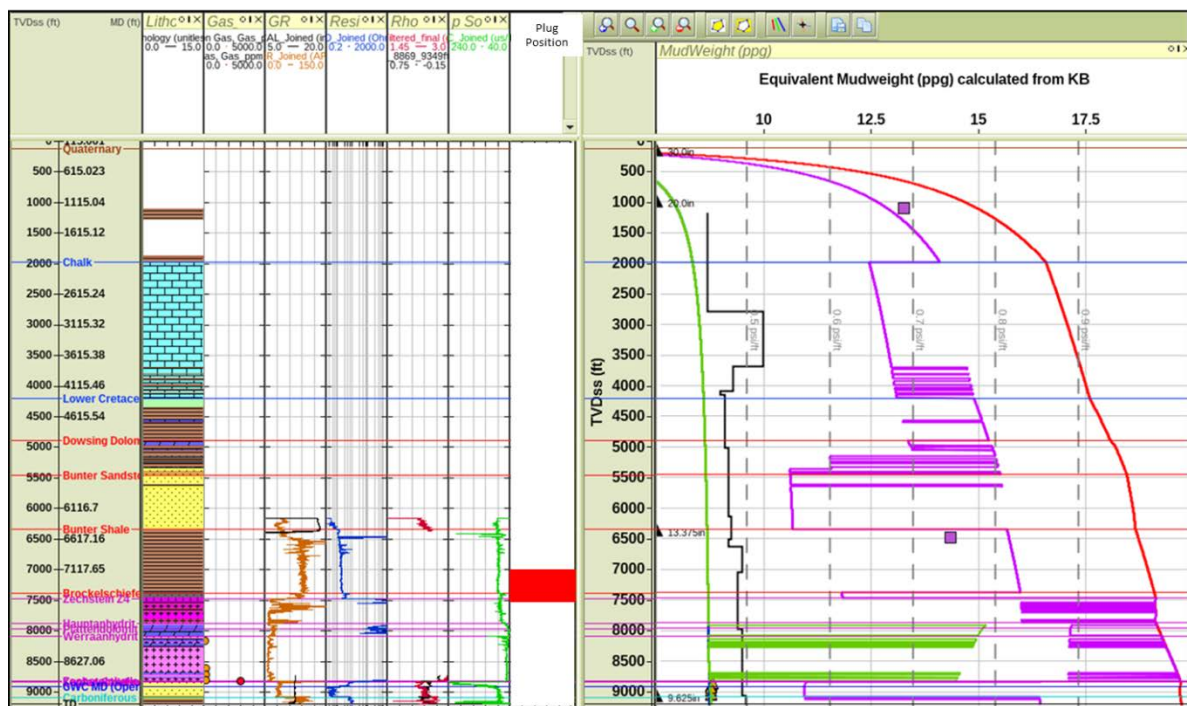
Figure 2: An example of a plug-plan summarising all the relevant geological, geophysical and drilling information to guide cement plug placement.
