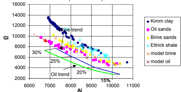
Figure 3. AIGI Crossplot
